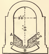
FIG. 7. OLD LONDON SEWER WITH IMPROVED INVERT.
